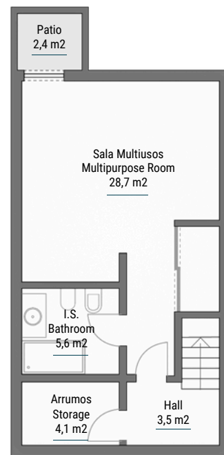
CAVE BASEMENT
